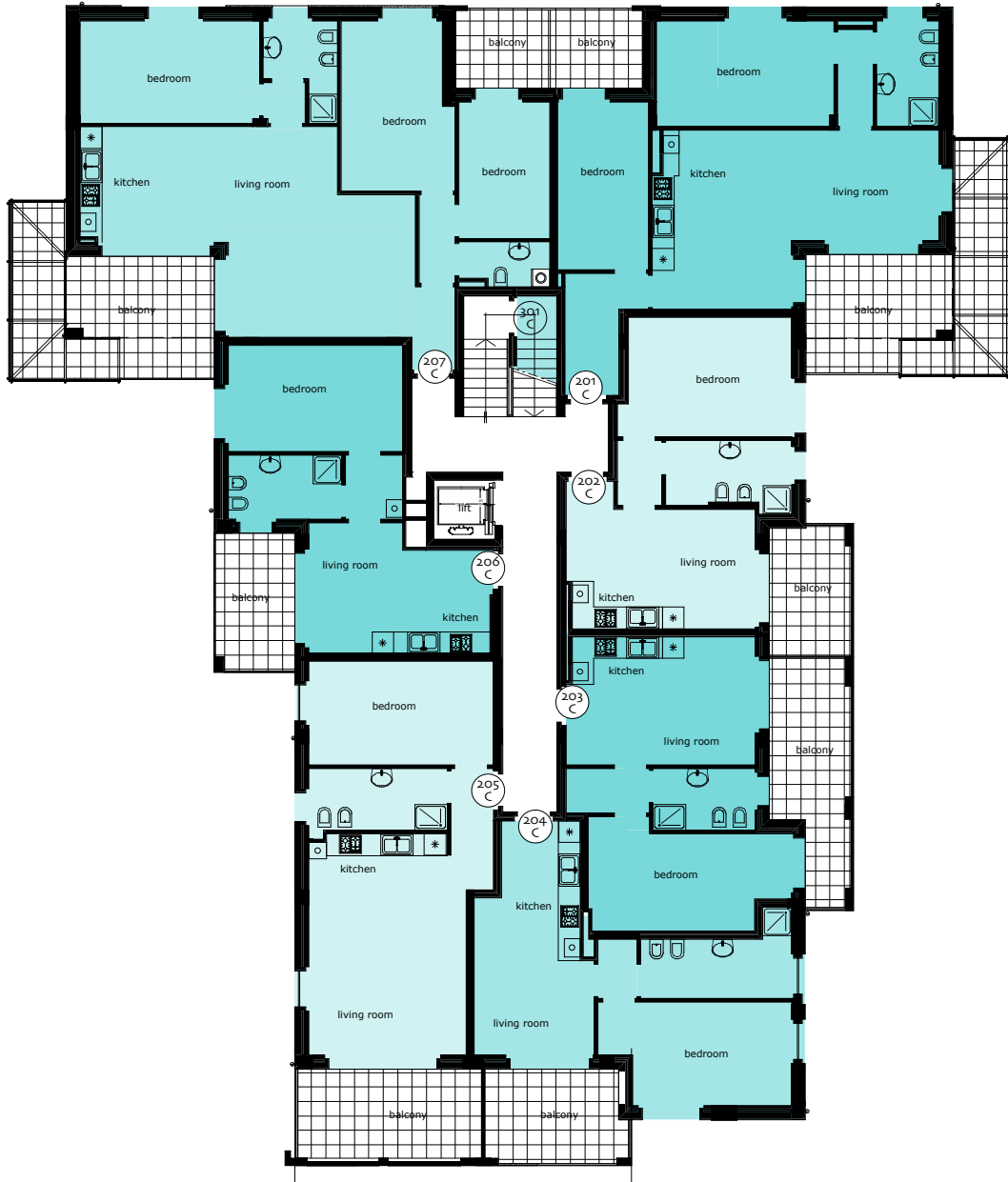
SECOND FLOOR
